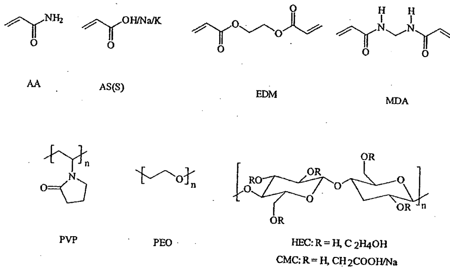
Fig. 2: Used monomers, cross-linkers and rheological additives
